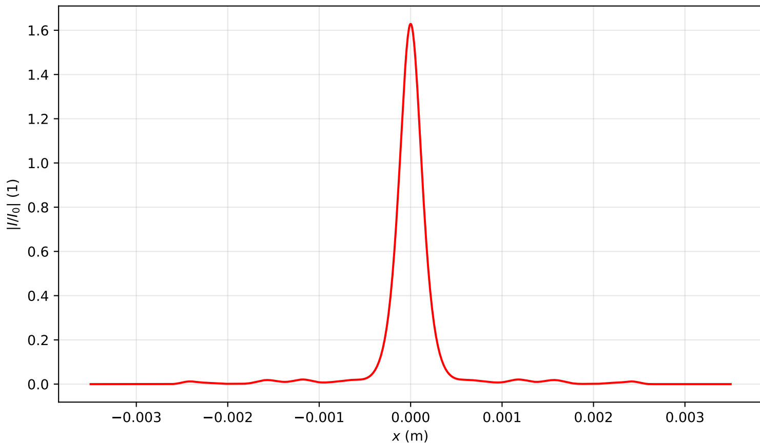
Intensity profile I(x, y = 0, z = 3.821)/I_0 , P_{in}=4.0P_{cr} , artificial time
